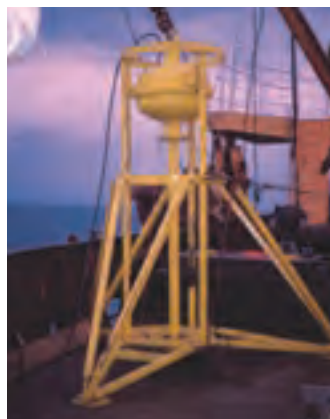
FIGURE 6 Vibrocorer
