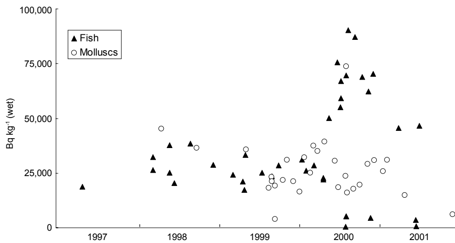
Figure 8.1 Tritium concentrations in fish and molluscs from Cardiff
