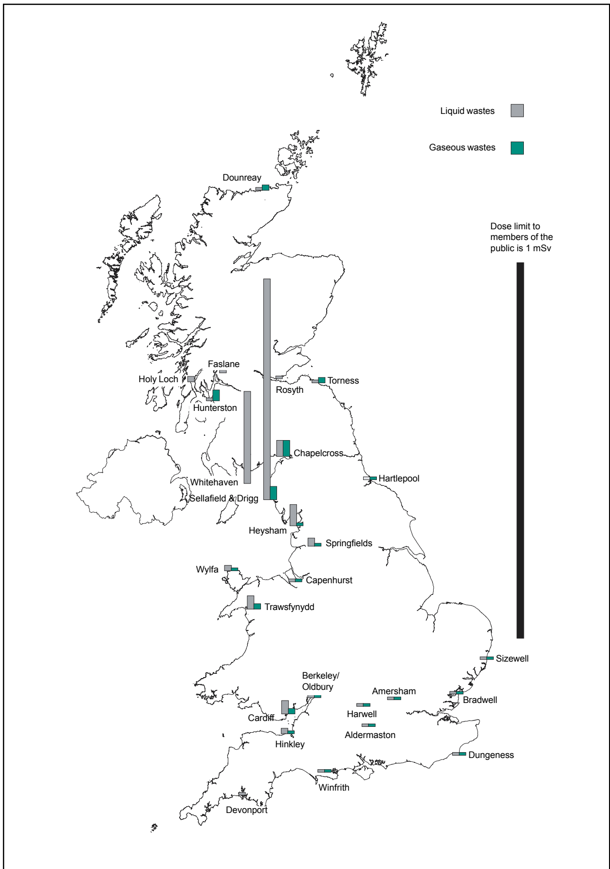
Figure S. Radiation exposures in the UK due to radioactive waste discharges, 2001 - Food Standards Agency and SEPA surveillance (Exposures at Whitehaven and Sellafield include the effects of artificial and enhanced natural nuclides from nuclear and non-nuclear industries)
