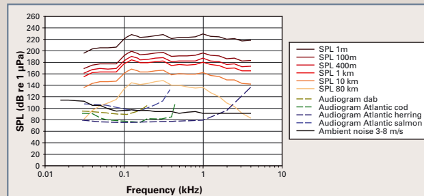
Figure 2: Attenuation of pile-driving noise at different distances from the source, ambient noise levels and audiograms of target fish species (Pile-driving noise after ITAP (2005) and Betke, pers. comm; values as dB 0-P re 1 µPa in 1/3 octave-bands; TL-calculations after Thiele (2002); ambient noise levels in 1/3 octave-bands in dB re 1 µPa after DEWI (2004); audiograms after Enger 1967; Chapman and Hawkins 1973; Chapman and Sand 1974; Hawkins and Johnstone 1978).
