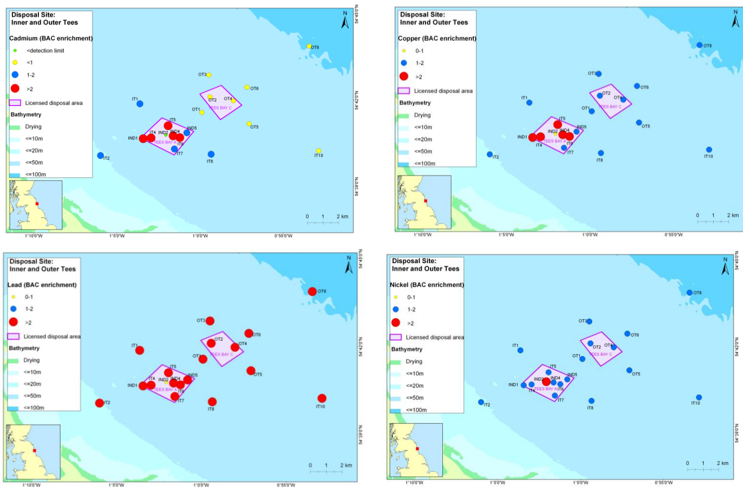
Figure 2.3.17 Enrichment to OSPAR BACs (raw/OSPAR BAC) at Tees (Inner and Outer) in 2009 for Cd, Cu, Pb and Ni.
