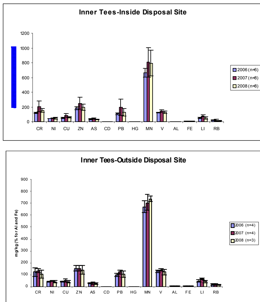
Figure 2.54. Concentrations of metals for stations inside (top) and outside (bottom) the Inner Tees disposal site between 2006 and 2008.
