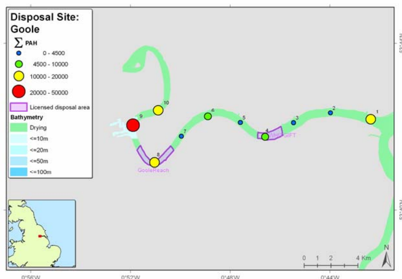
Figure 2.65. Summed PAH concentrations for the Goole stations, 2008.
