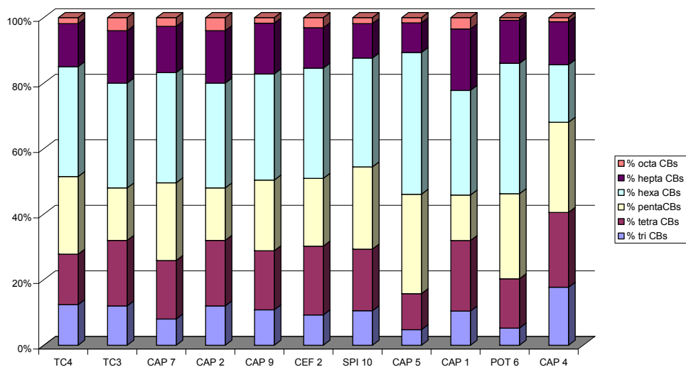
Figure 2.27. CB congener profiles for the Souter Point stations, 2008.
