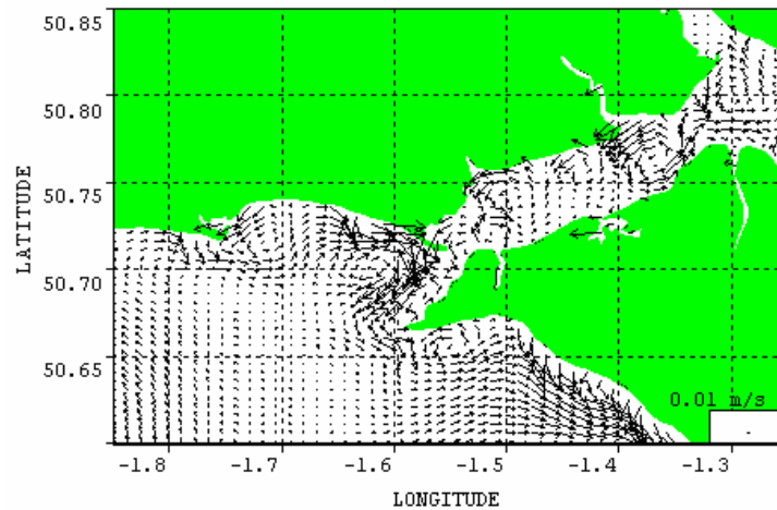
Figure 2.81. Residual flow for the region.
