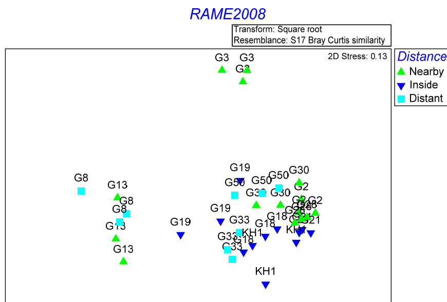
Figure 2.87. MDS plot of samples (labels) and distance from disposal site (symbols). ANOSIM results show that samples from the same site are similar ( R=0.835 P=0.1\% ) but that the variation is not a factor of distance ( R=0.171 P=0.7\% ).
