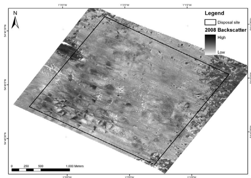
Figure 2.35. Inner Tees seabed backscatter from the 2008 multibeam echosounder survey.
