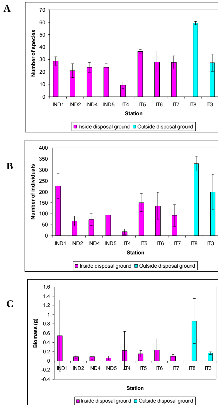
Figure 2.40A-C. Inner Tees Bay. A. Mean number of species (+/- standard deviation). B. Mean number of individuals (+/- standard deviation). C. Mean biomass (+/- standard deviation).
