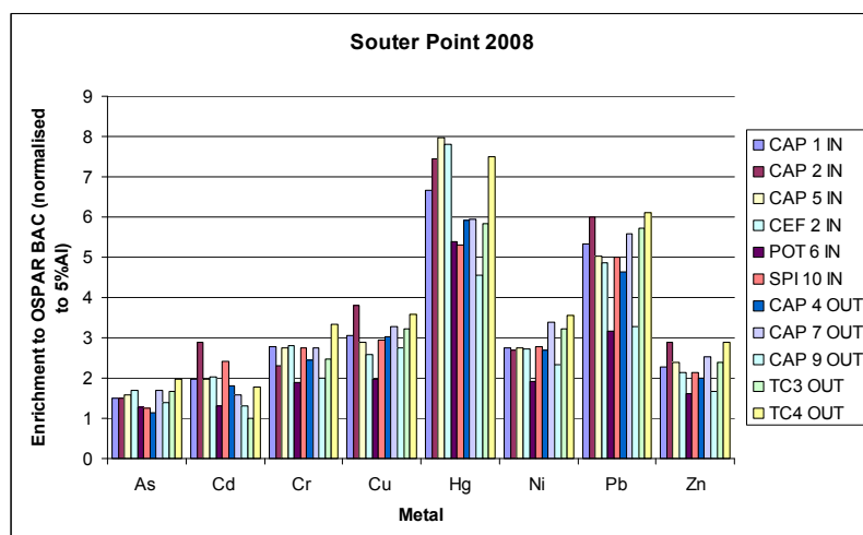
Figure 2.31. Enrichment to OSPAR BACs for metal concentrations measured at Souter Point in 2006 (top), 2007 (middle), and 2008 (bottom).
