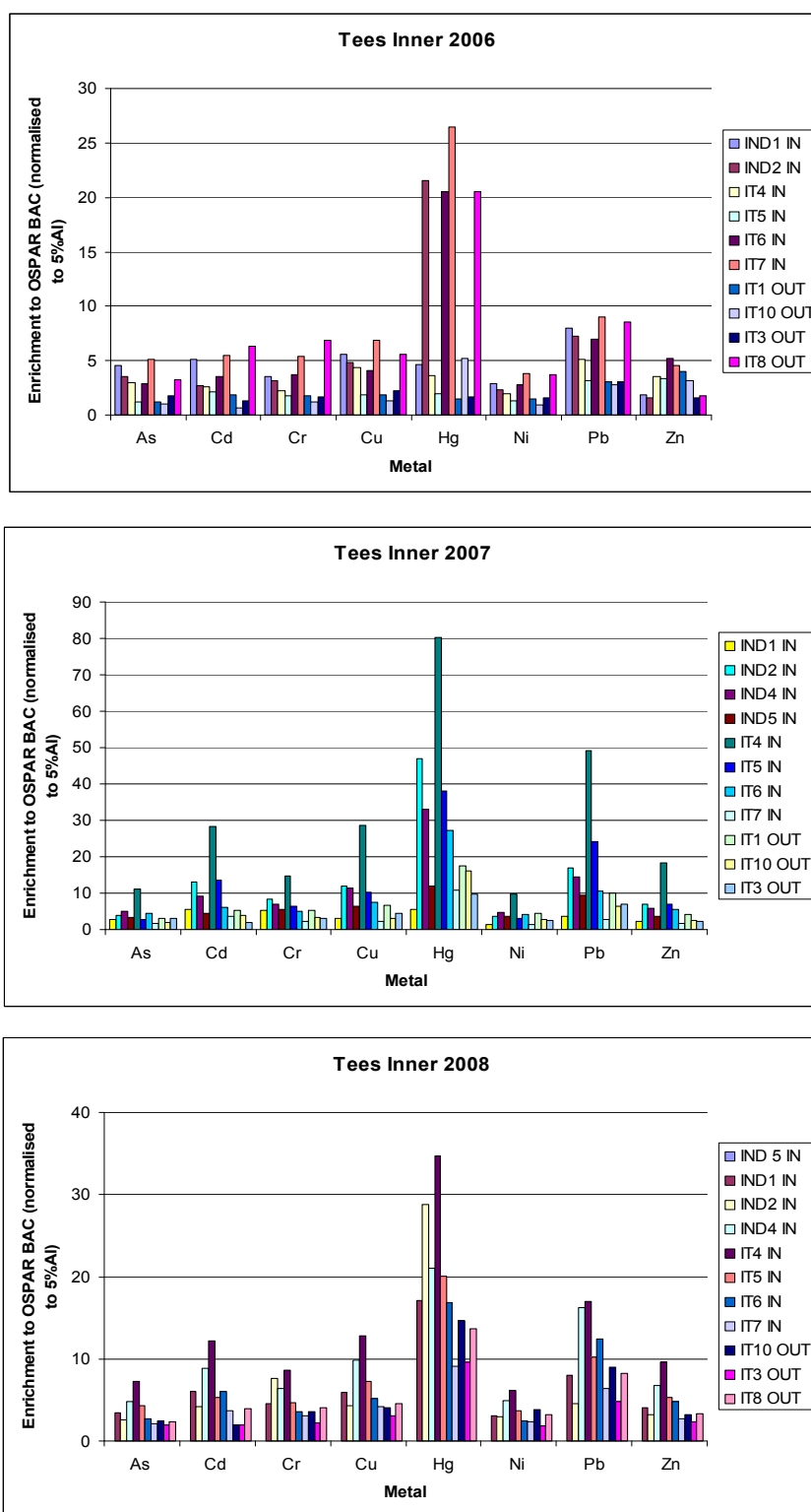
Figure 2.55. Enrichment to OSPAR BACs for metal concentrations measured at Inner Tees in 2006 (top), 2007 (middle), and 2008 (bottom).
