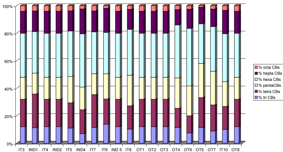
Figure 2.47. CB congener profiles for the Inner and Outer Tees stations, 2008.
