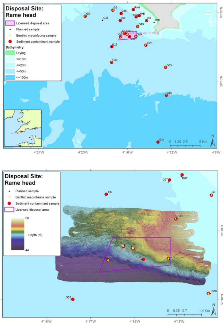
Figure 2.82. Locations of all monitoring stations for Rame Head, 2008 (top), and stations closer to the disposal site with the multibeam image from 2007 superimposed (bottom).
