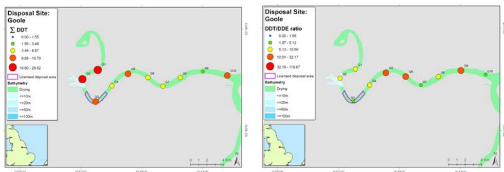
Figure 2.70. Summed DDT concentrations (left) and DDT / DDE ratios (right) for the Goole stations, 2008.
