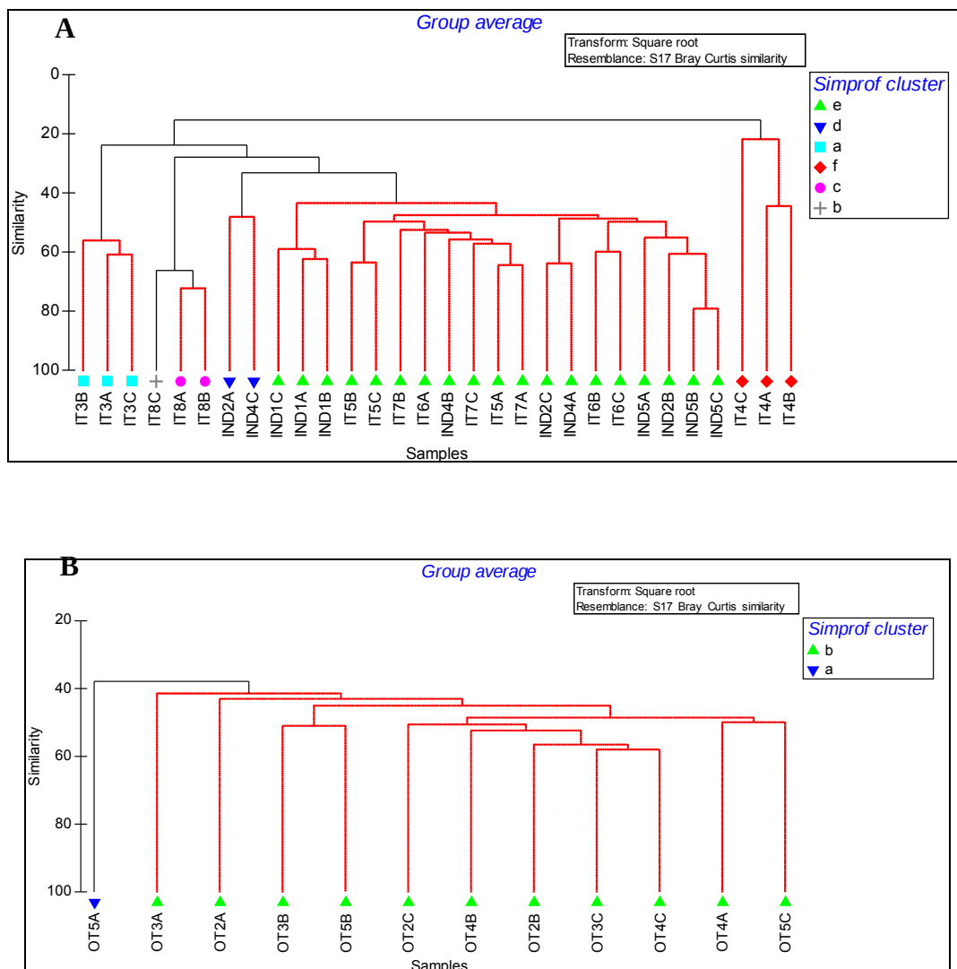
Figure 2.42. Hierarchical cluster analysis with a SIMPROF test (significance level 5%) of abundance data for A) Inner Tees Bay, and B) Outer Tees Bay.
