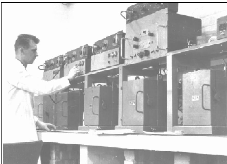
Figure 5. Ian Huggins with the bank of shielded GM detectors for beta counting. Note the stop-watches in use. The scalers such as being operated by Ian were transistorised and built in-house
